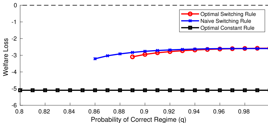
Fig. 4. Monetary policy errors and relative welfare loss.
