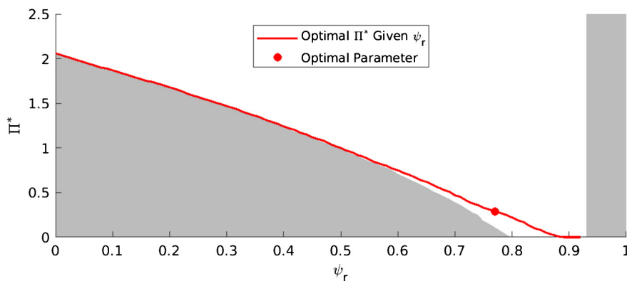
Fig. 2. Optimal constant rules with regime switching.
