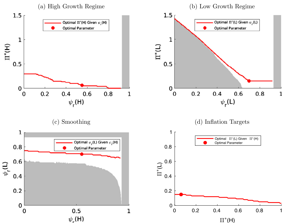
Fig. 3. Optimal switching rules with regime switching.
