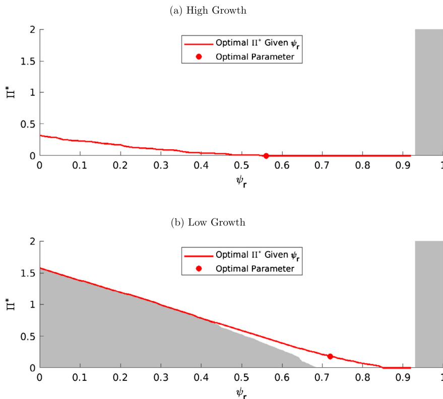
Fig. 1. Optimal rules without regime switching.
